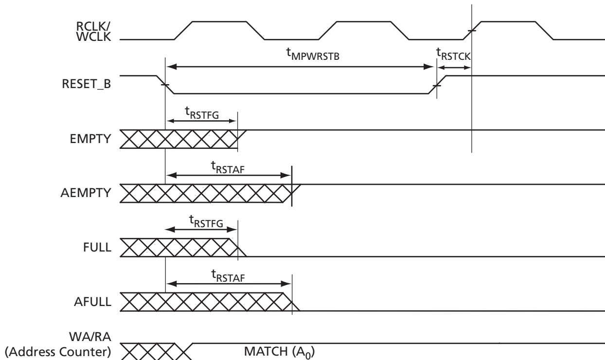
Figure 2-52 • FIFO Reset
