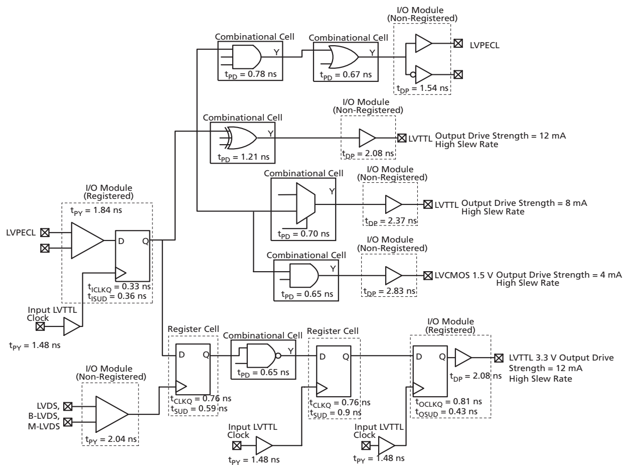
Figure 2-4 • Timing Model
