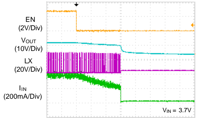
Time (5ms/Div)
