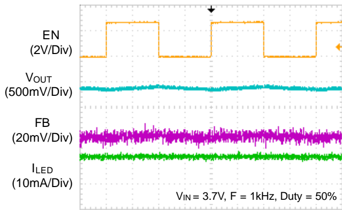
Time (250μs/Div)
