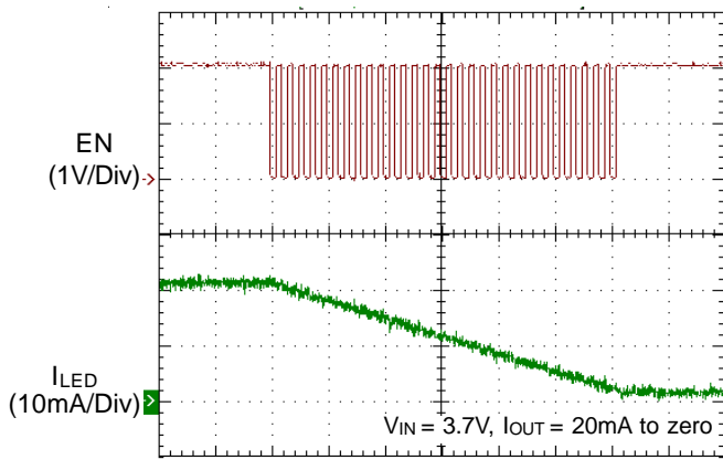
Time (5ms/Div)
