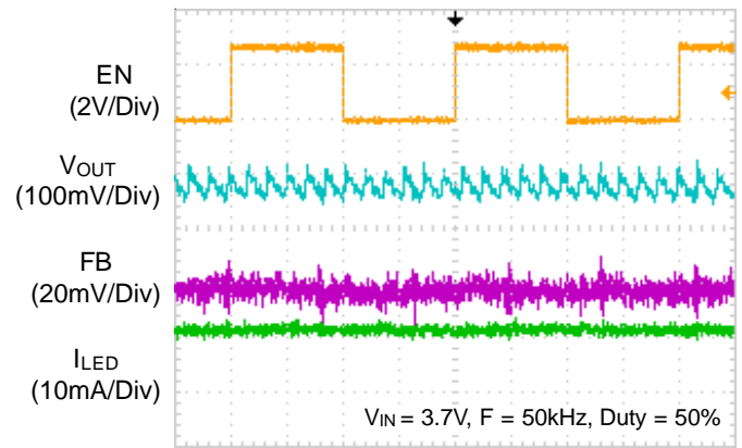
Time (5μs/Div)
