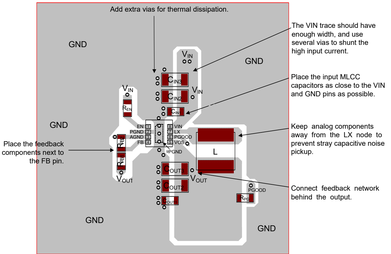
Figure 4. PCB Layout Guide
