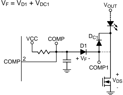
Figure 3. COMP Circuit
