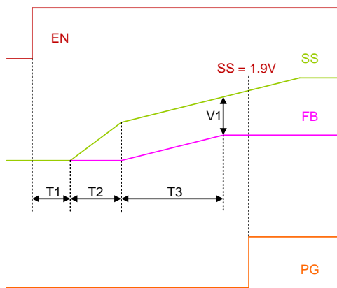
T1 : EN delay, from EN go high to SS start rising, T1 = 50µs; T2 : speed up SS, from SS rising to FB start rising, T2 = C SS × 0.7/30µA; T3 : normal SS, from FB rising to settled, T3 = C SS × V FB /I SS ; V1 : offset voltage between SS and FB, V1 = 700mV; PG go high after SSOK (SS = 1.9V)
