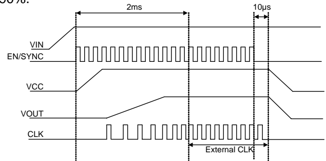
Figure 6. Startup Sequence Using External Sync Clock
