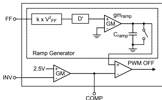
Figure 10. Ramp Generator
