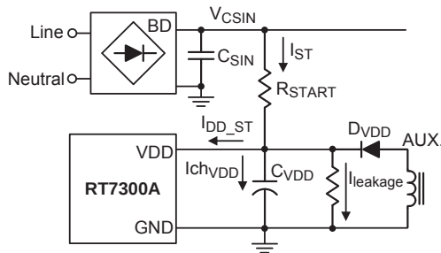
Figure 11. Start-Up Circuit
