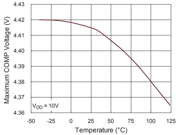
Maximum COMP Voltage vs. Temperature
