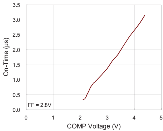
On-Time vs. COMP Voltage
