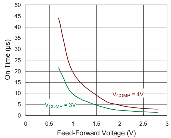
On-Time vs. Feed-Forward Voltage
