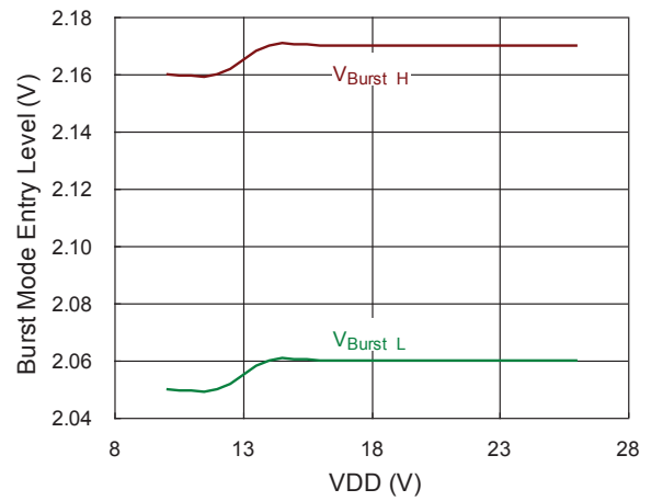
Burst Mode Entry Level vs. VDD
