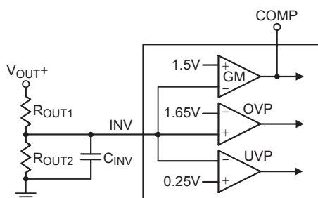
Figure 5. Feedback Voltage Detection
