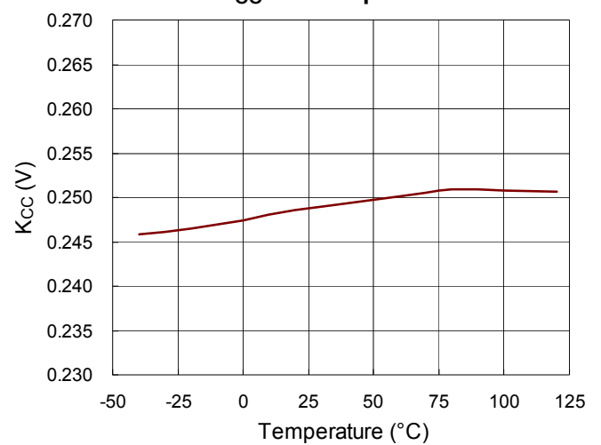
K_{CC} vs. Temperature
