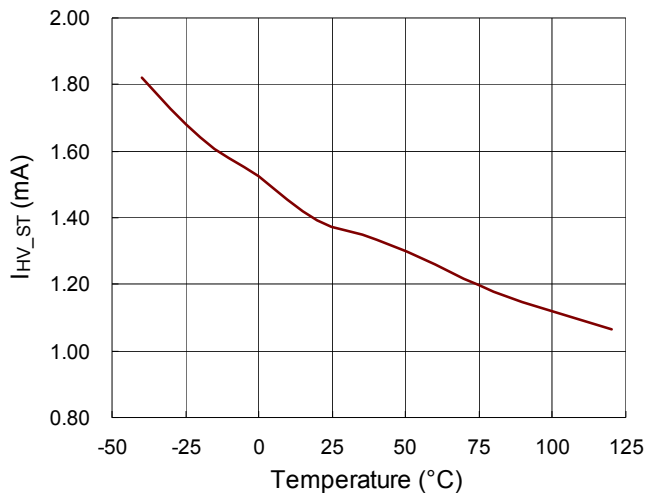
I_{HV\_ST} vs. Temperature
