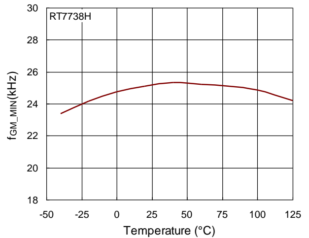
f GM_MIN vs. Temperature
