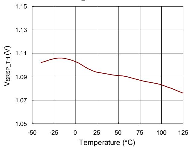
V SRSP_TH vs. Temperature
