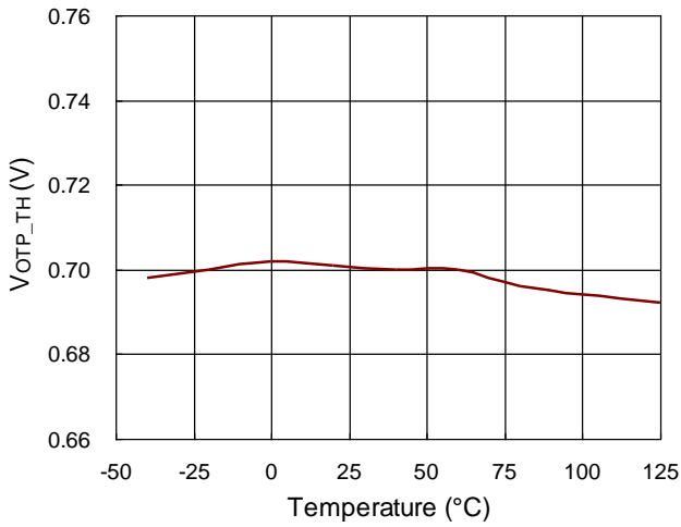
V OTP_TH vs. Temperature
