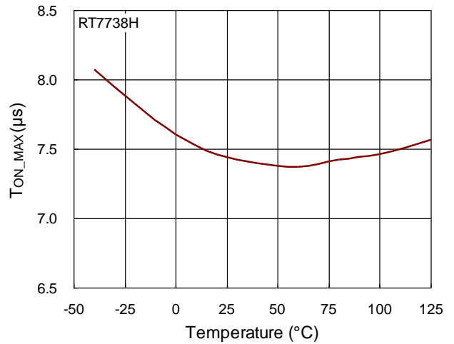
T ON_MAX vs. Temperature
