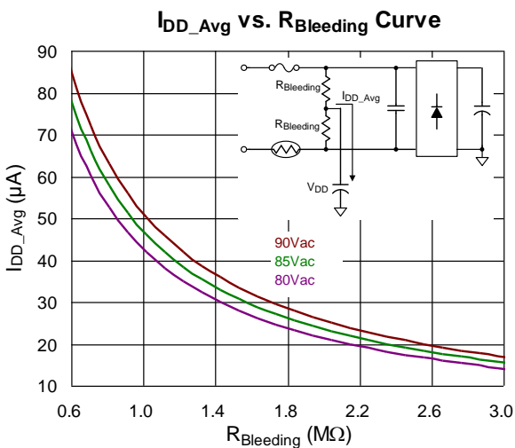
Figure 7. I DD_Avg vs. R Bleeding Curve
