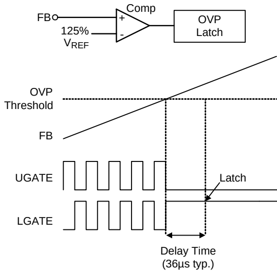
Figure 4. OVP Operation
