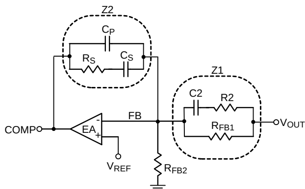
Figure 6. Type-III Compensator
