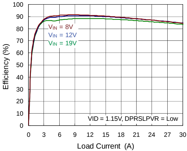
CCM Efficiency vs. Load Current
