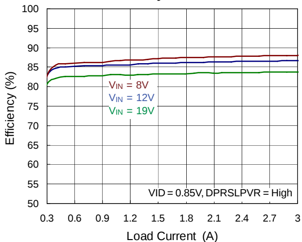
RFM Efficiency vs. Load Current
