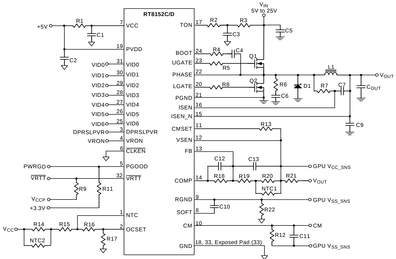
Figure 2. Render Core Voltage Regulator
