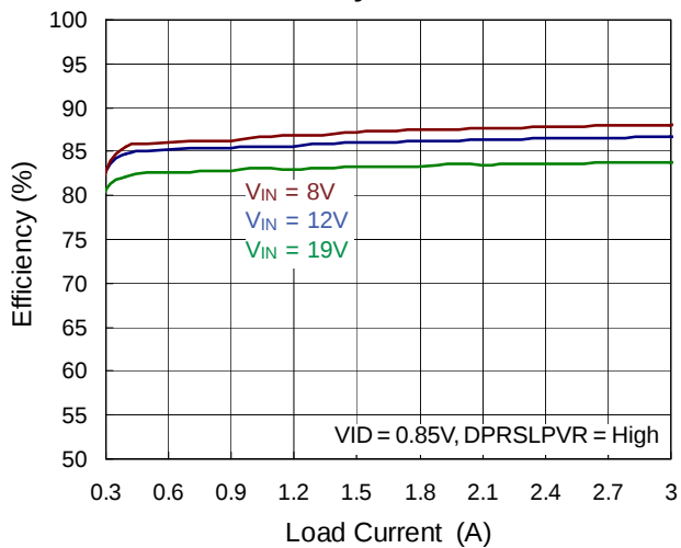
RFM Efficiency vs. Load Current
