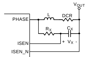
Figure 3. Lossless Inductor Current Sensing
