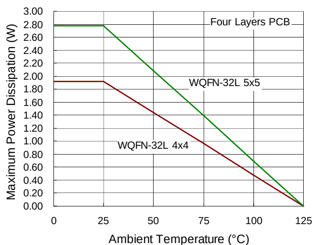
Figure 17. Derating Curve for RT8153C/D Package
