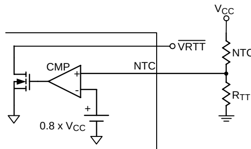
Figure 14. Thermal Throttling Setting Principle
