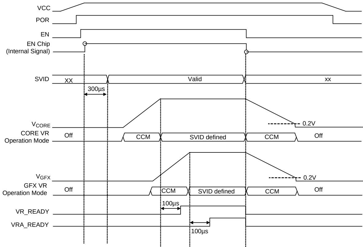
Figure 7 (a). Power sequence for RT8165B ( V_{INI\_CORE} = V_{INI\_GFX} = 0V )
