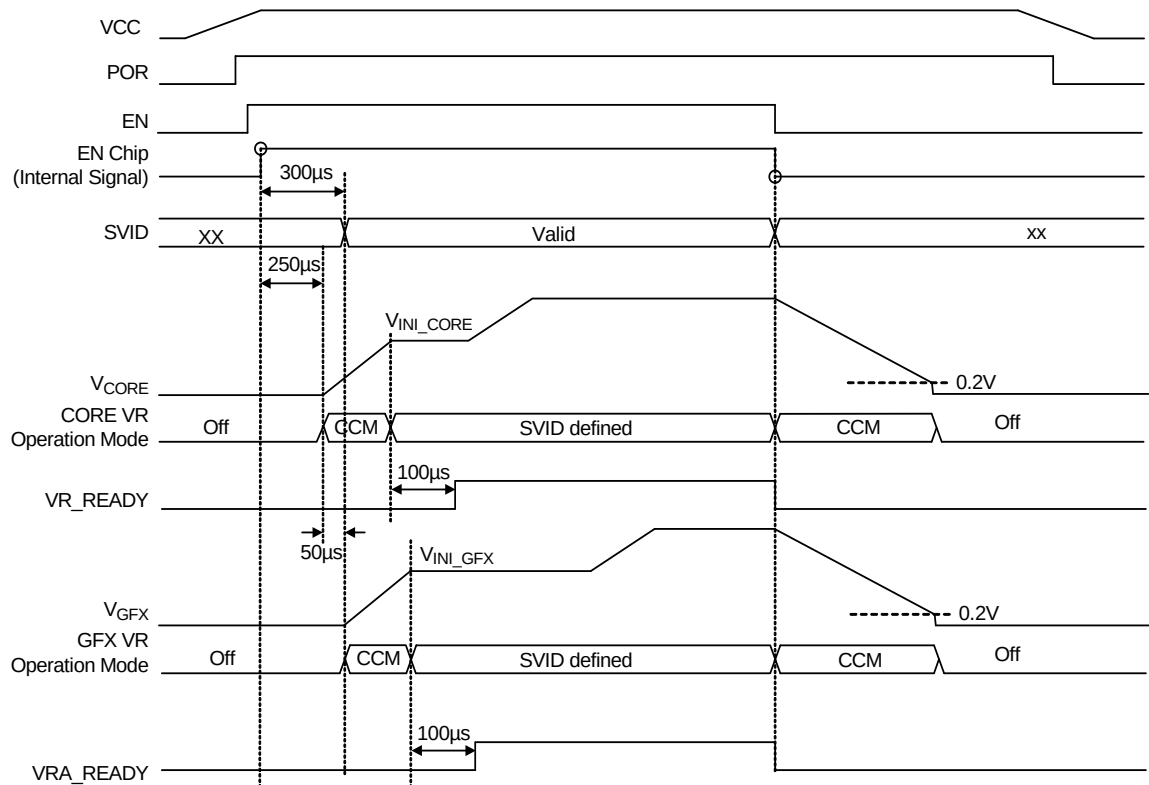
Figure 7 (b). Power sequence for RT8165B ( V_{INI\_CORE} \neq 0 , V_{INI\_GFX} \neq 0V )
