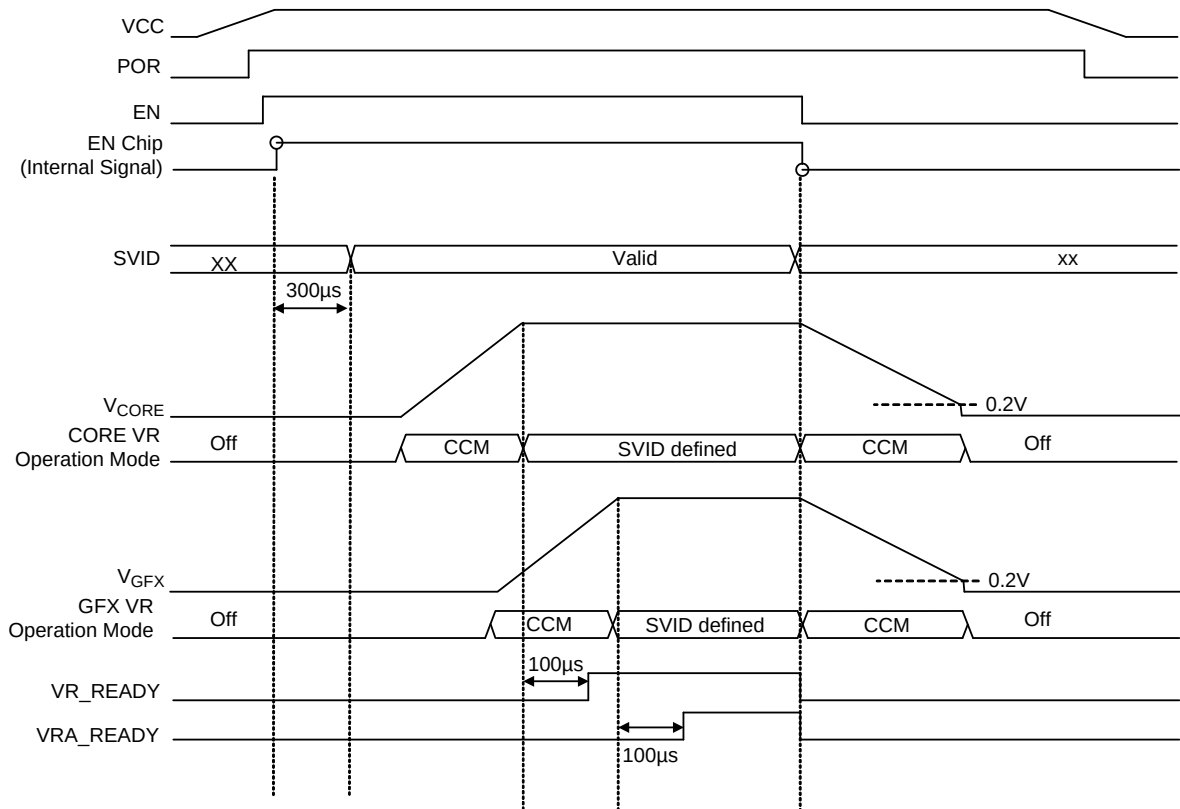
Figure 5 (a). Power sequence for RT8166B ( V_{INI\_CORE} = V_{INI\_GFX} = 0V )
