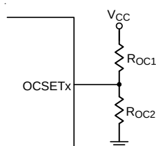
Figure 12. OCP Setting without Temperature Compensation
