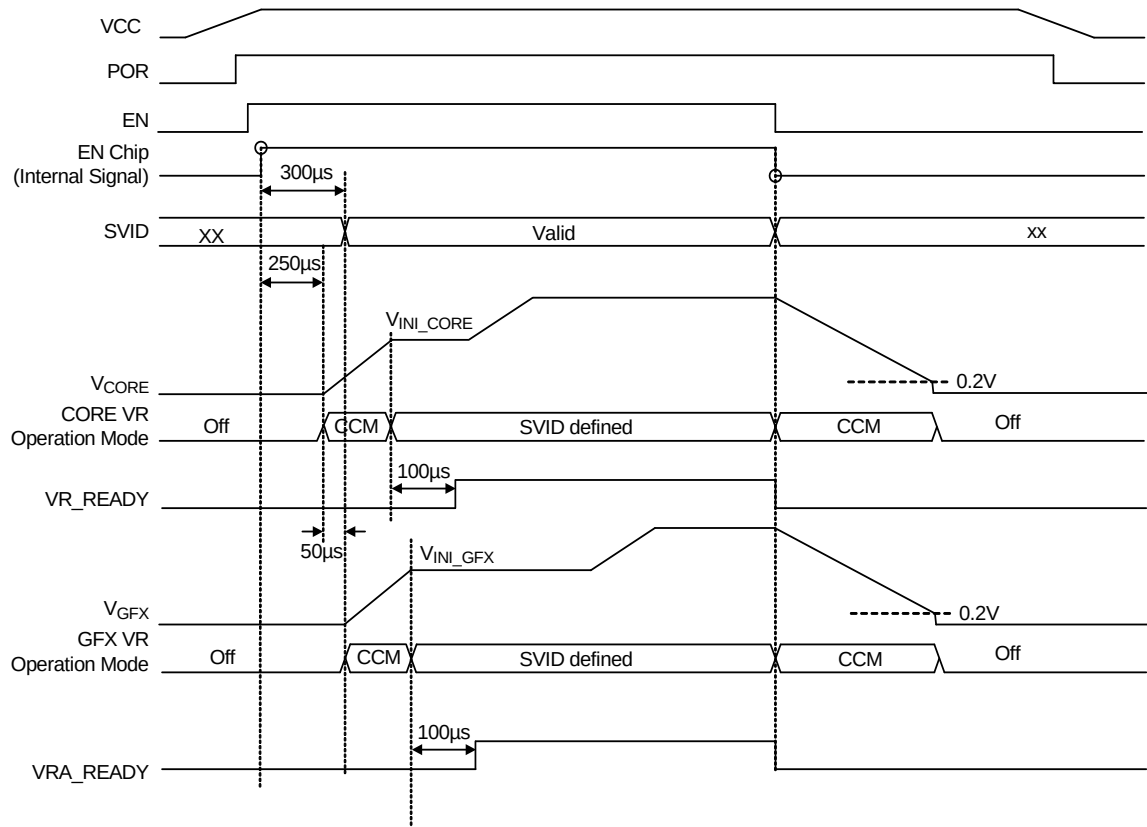
Figure 5 (b). Power sequence for RT8166B ( V_{INI\_CORE} \neq 0 , V_{INI\_GFX} \neq 0V )
