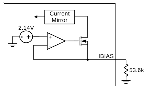
Figure 4. IBIAS Setting
