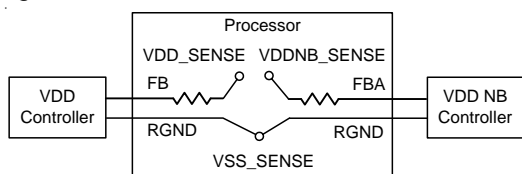
Figure 5. Differential Remote Voltage Sense Connection
