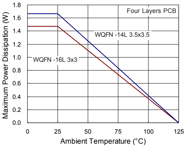
Figure 5. Derating Curves for RT8209L/M Packages
