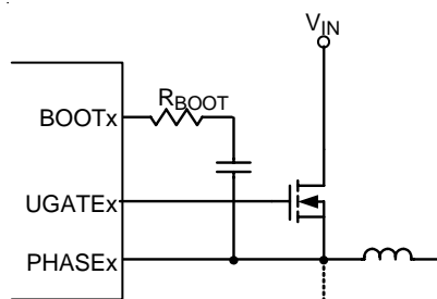
Figure 3. Reducing the UGATEx Rise Time
