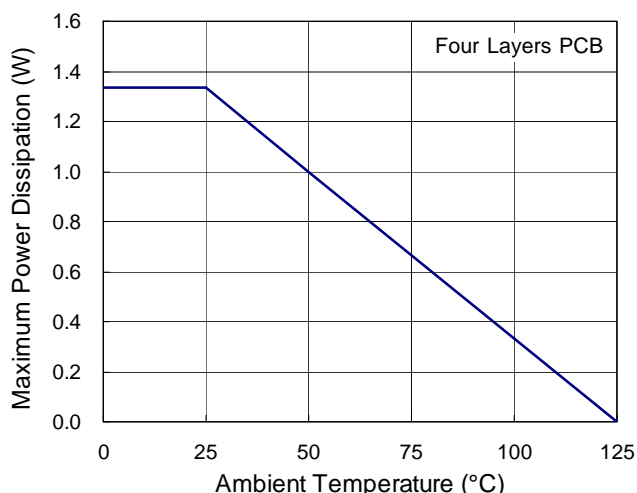
Figure 3. Derating Curve for RT8274 Package
