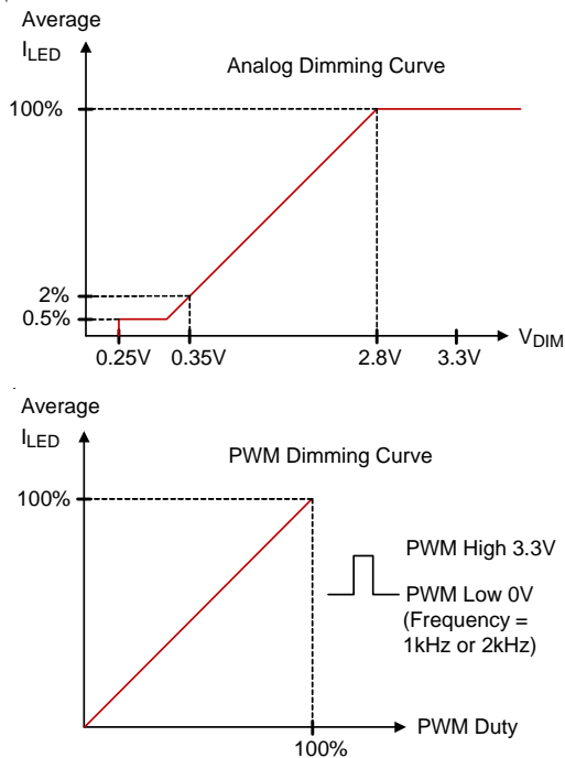
Figure 1. Dimming Curve
