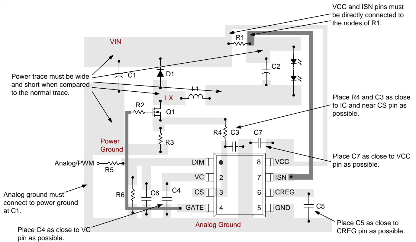
Figure 3. PCB Layout Guide
