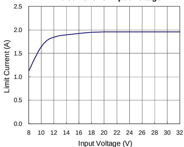
Limit Current vs. Input Voltage
