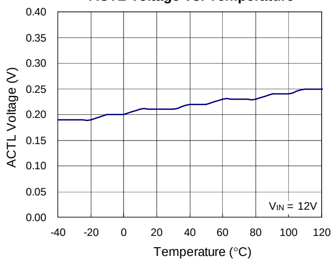
ACTL Voltage vs. Temperature
