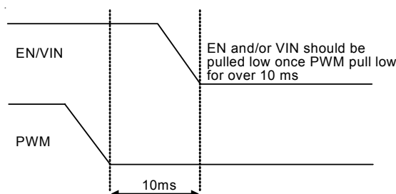
Figure 6. To Prevent "Hard-Start" Sequence
