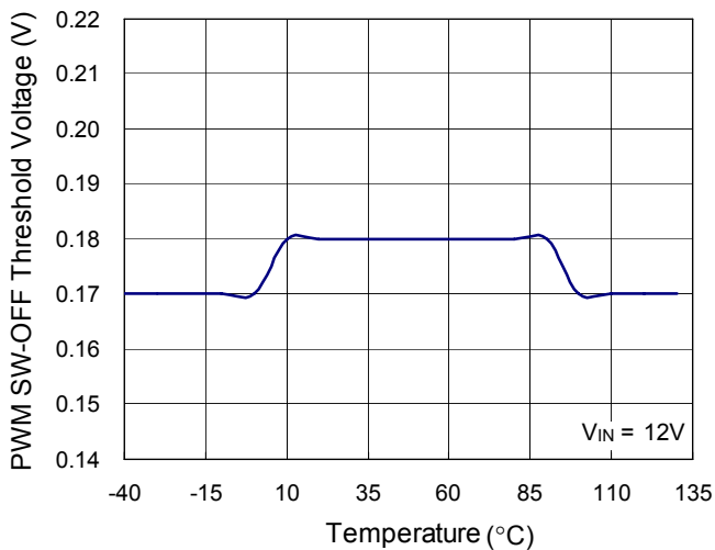
PWM SW-OFF Threshold Voltage vs. Temperature
