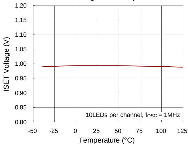
ISSET Voltage vs. Temperature
