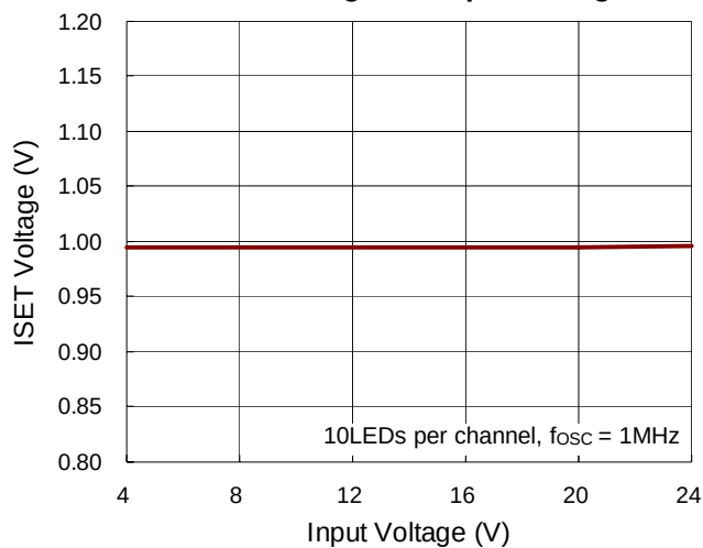
ISSET Voltage vs. Input Voltage
