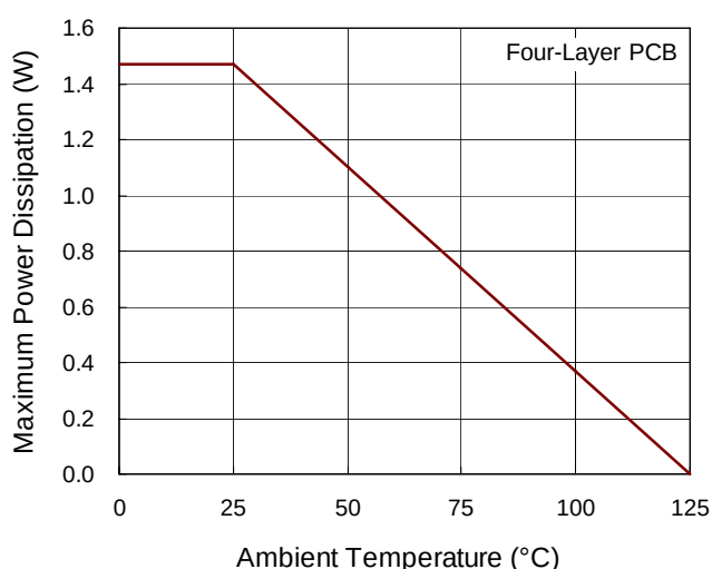
Figure 2. Derating Curve for RT8567 Package
