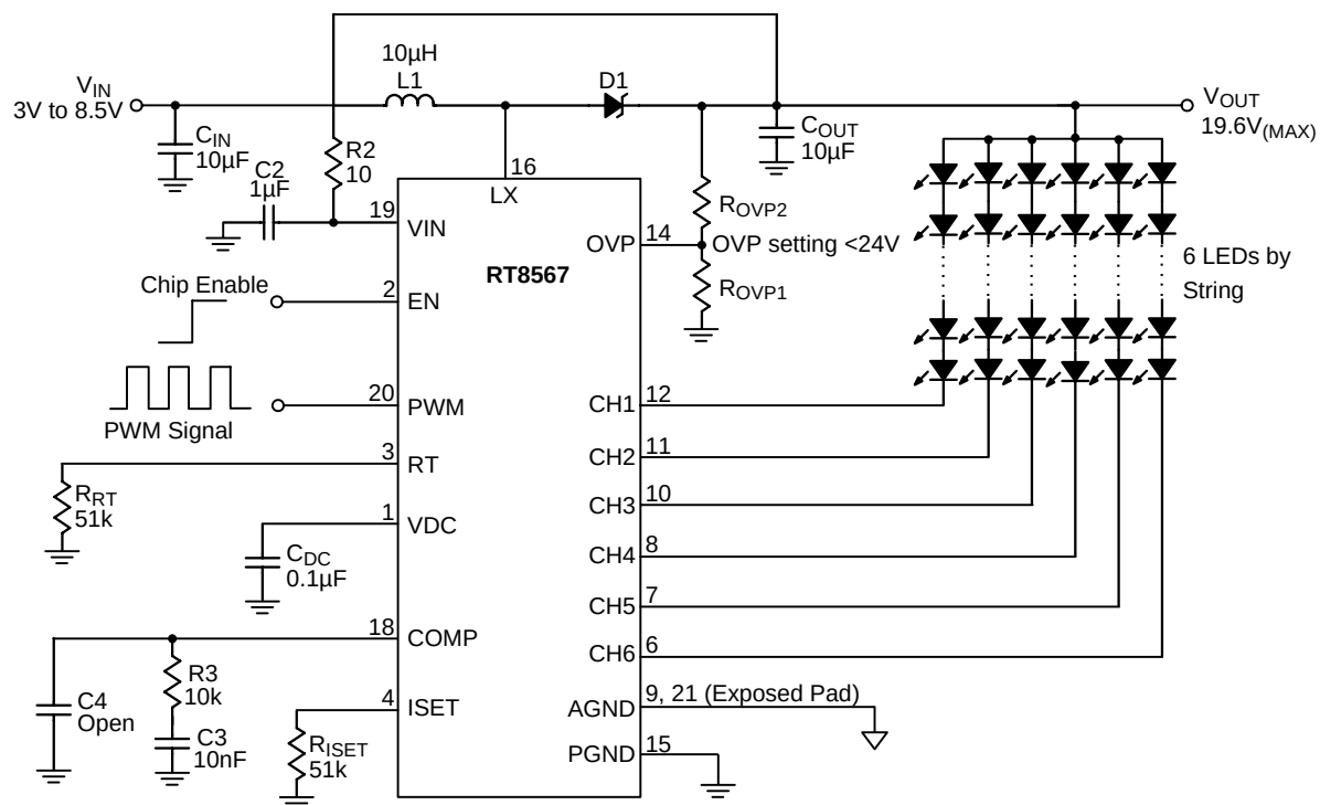
Figure 1. Application Circuit 1
