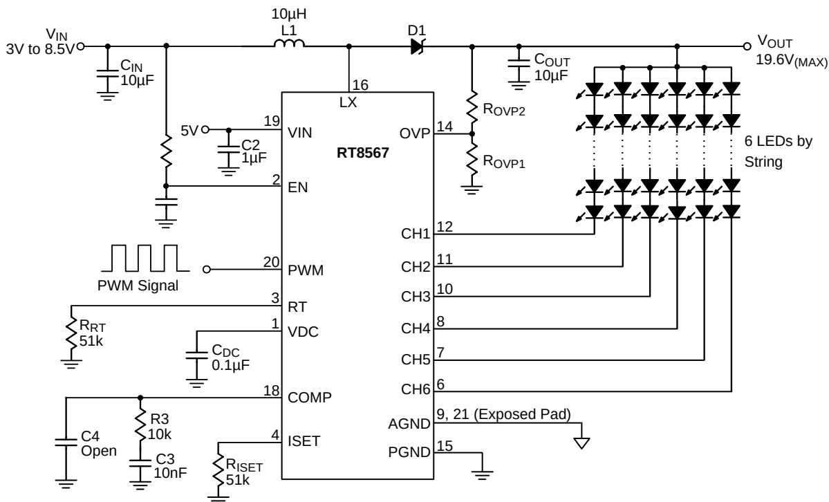
Figure 3. Application Circuit 3
