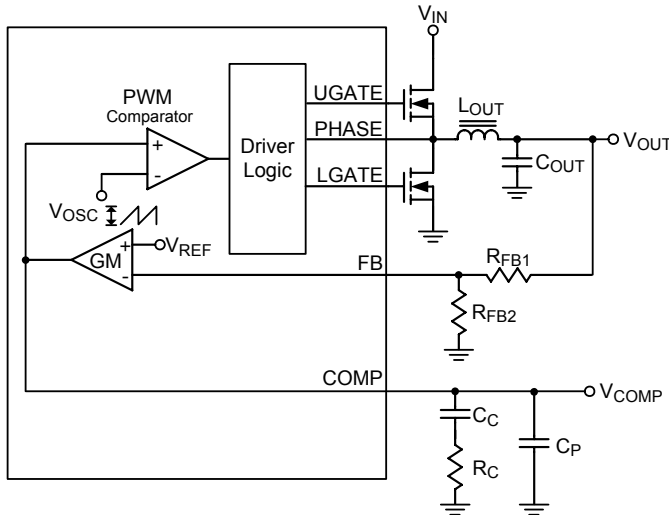
Figure 9. Typical Voltage Mode Buck Converter Control Loop
