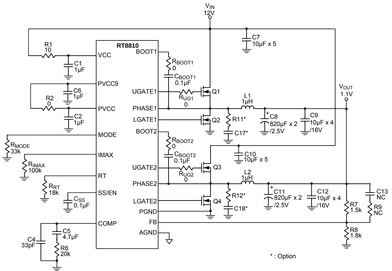
Figure 2. RT8810B
