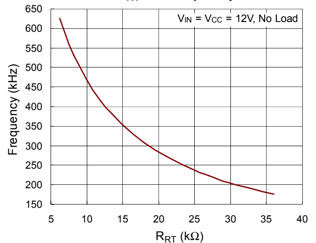
R_{RT} vs. Frequency
