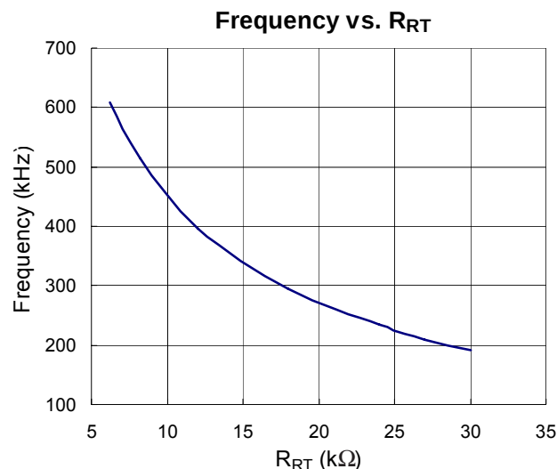
Figure 4. R_{RT} vs. Switching Frequency
