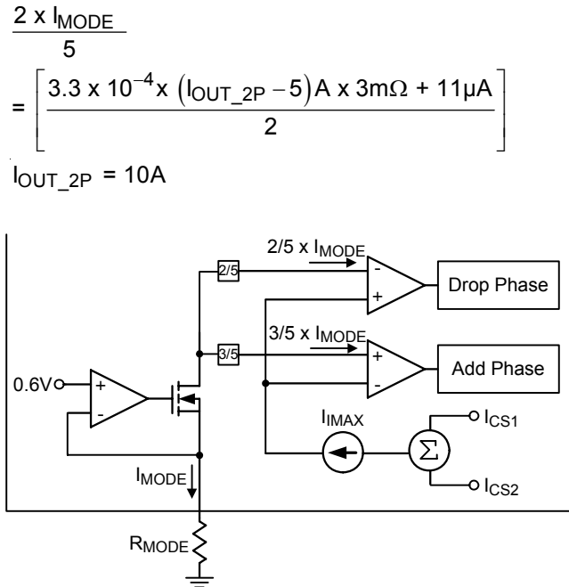
Figure 6. Dynamic Phase Number Control Circuit
