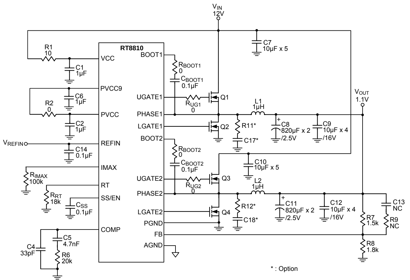
Figure 3. RT8810C
