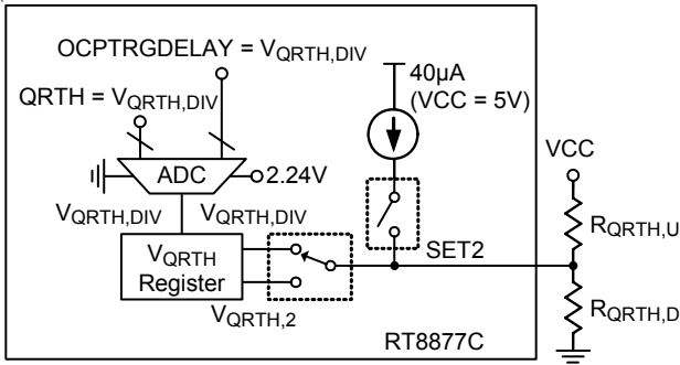
Figure 7. QRTH/OCPTRGDELAY Setting
