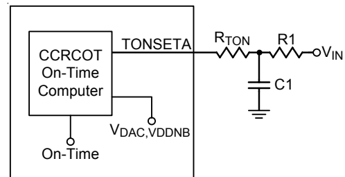
Figure 18. VDDNB Controller : On-Time Setting with R C Filter
