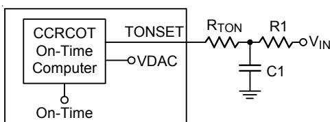
Figure 11. VDD Controller : On-Time Setting with R_C filter
