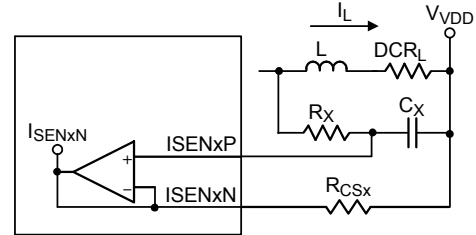
Figure 12. VDD Controller : Lossless Inductor Sensing
