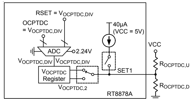
Figure 6. OCP_TDC/RSET Setting
