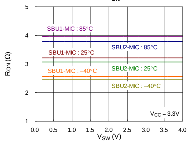
MIC Switch R_{ON} Flatness
