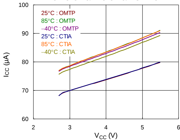
Supply Current - AUDIO On & MIC On & AGND On
