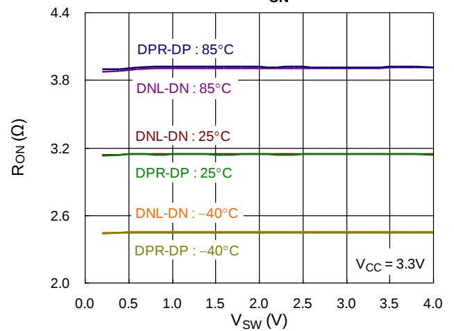
USB Switch R_{ON} Flatness
