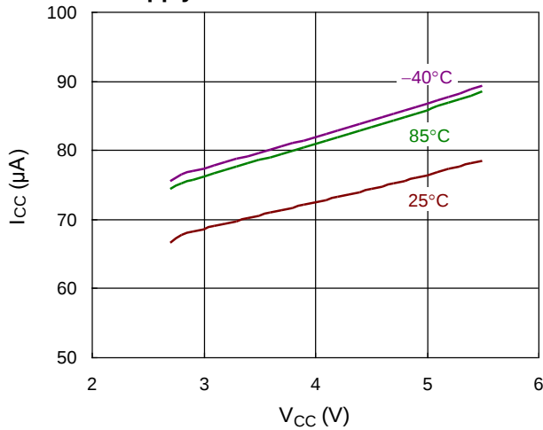
Supply Current - USB On &amp; SBU On
