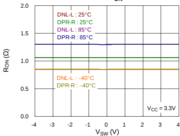
AUDIO Switch R_{ON} Flatness
