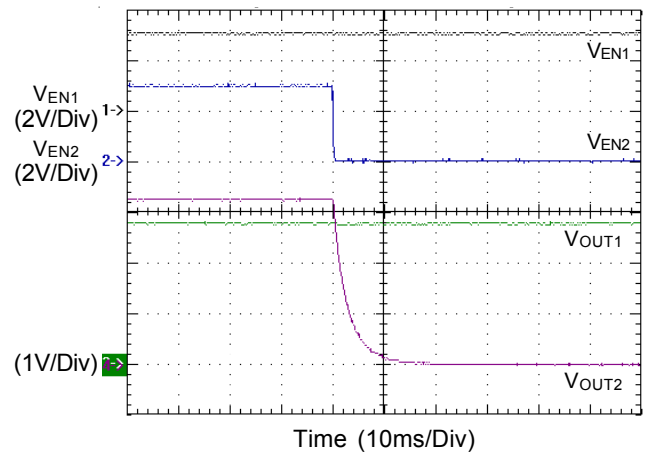
EN2 Pin Shutdown Response
