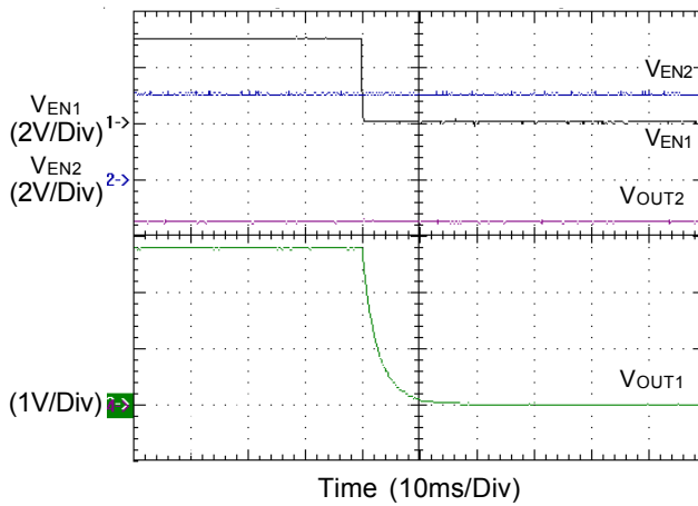
EN1 Pin Shutdown Response
