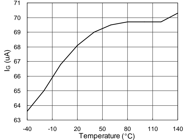
GND Current vs. Temperature
