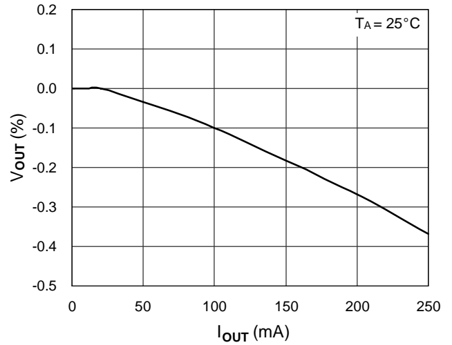
Output Voltage Variation vs. Load
