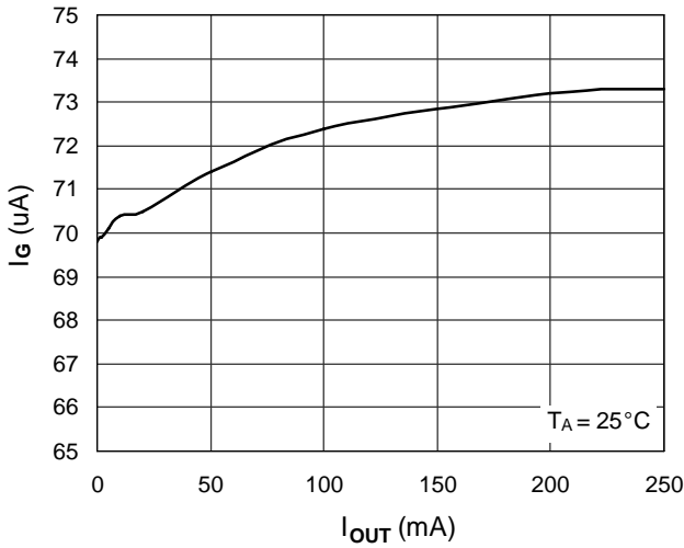
Quiescent Current vs. Load
