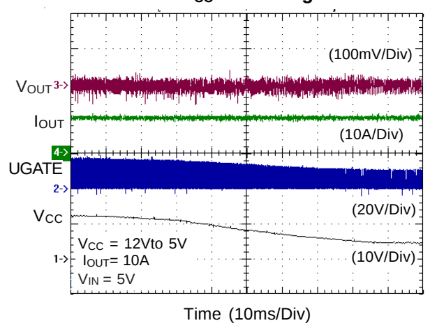
VCC Switching
