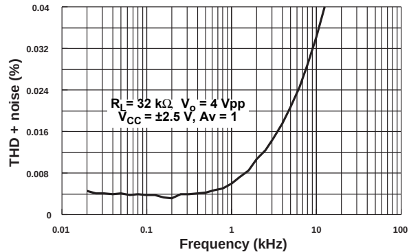
Figure 6. THD + noise vs. frequency ( R_L = 32\text{ }\Omega , V_o = 4\text{ Vpp} , V_{CC} = \pm 2.5\text{ V} )
