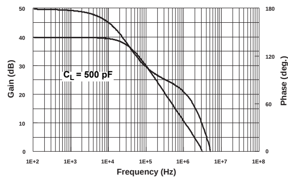
Figure 11. Open loop gain and phase vs. frequency
