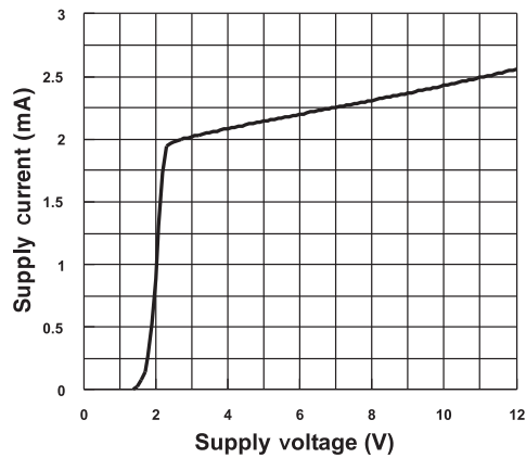
Figure 2. Total supply current vs. supply voltage
