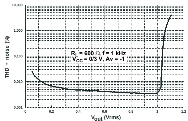
Figure 8. THD + noise vs. output voltage (R_L = 600\ \Omega, f = 1\text{ kHz}, V_{CC} = 0/3\text{ V})
