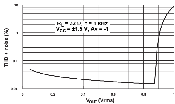
Figure 9. THD + noise vs. output voltage (R_L = 32\ \Omega, f = 1\text{ kHz}, V_{CC} = \pm 1.5\text{ V})
