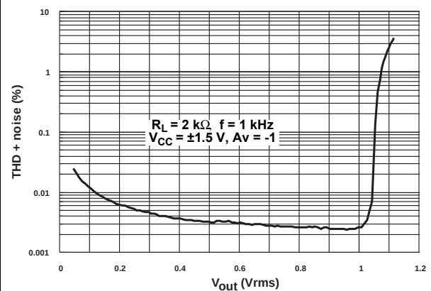
Figure 10. THD + noise vs. output voltage (R_L = 2\text{ k}\Omega, f = 1\text{ kHz}, V_{CC} = \pm 1.5\text{ V})
