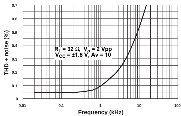
Figure 7. THD + noise vs. frequency (R_L = 32\ \Omega, V_o = 2\text{ Vpp}, V_{CC} = \pm 1.5\text{ V})
