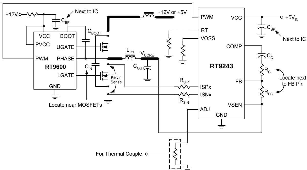
Figure 8. Layout Consideration
