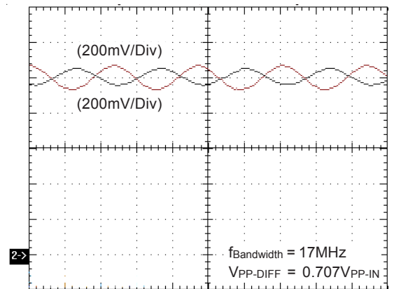
The Bandwidth of Differential Amplifier
