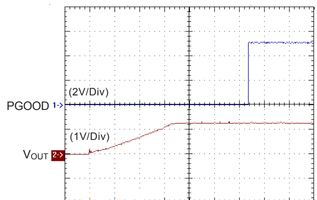
PGOOD Waveform
