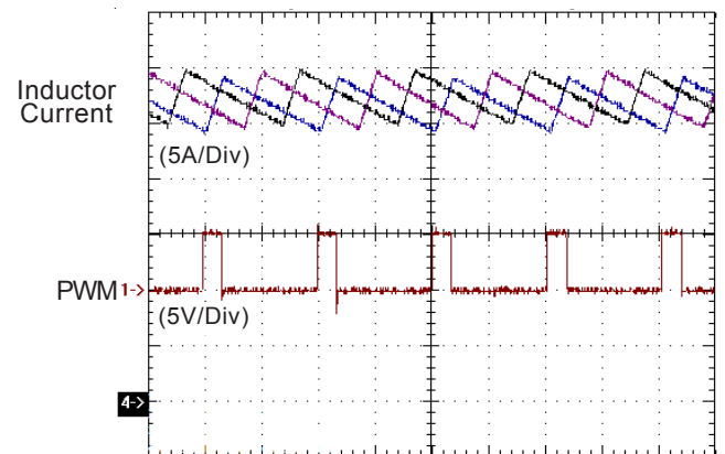
Current Sharing at I_{\text{OUT}} = 80\text{A}
