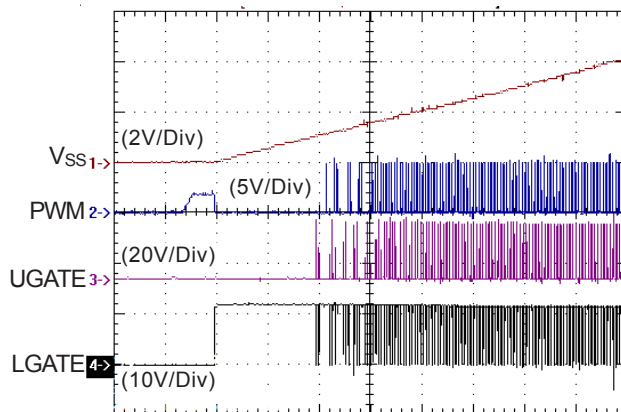
Start-up Waveforms @ I_{\text{OUT}} = 60\text{A}
