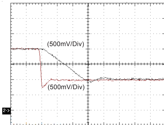
Differential Amp Falling Slew Rate
