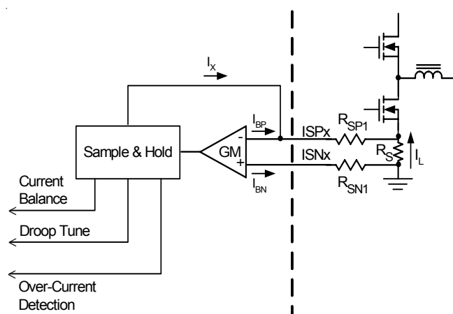
Figure 1. Current Sense Circuit
