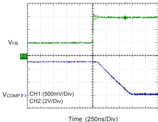
Figure 24. EA Rising Transient with 10pF Loading; Slew Rate = 8V/us
