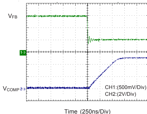
Figure 25. EA Falling Transient with 10pF Loading; Slew Rate = 8V/us
