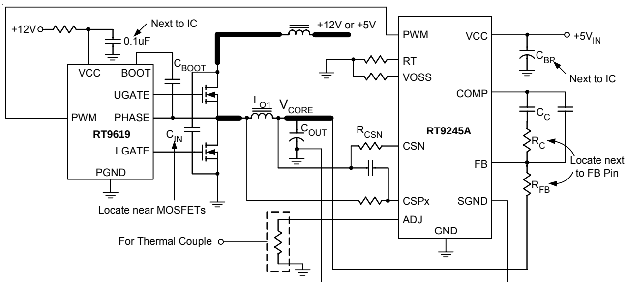
Figure 33. Layout Consideration
