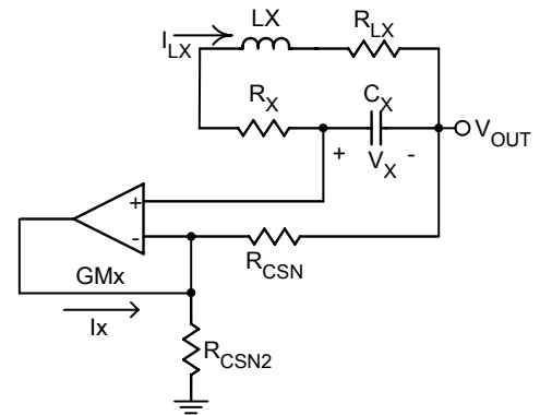
Figure 15. Application circuit of GM
