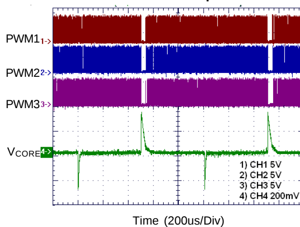
Transient Response
