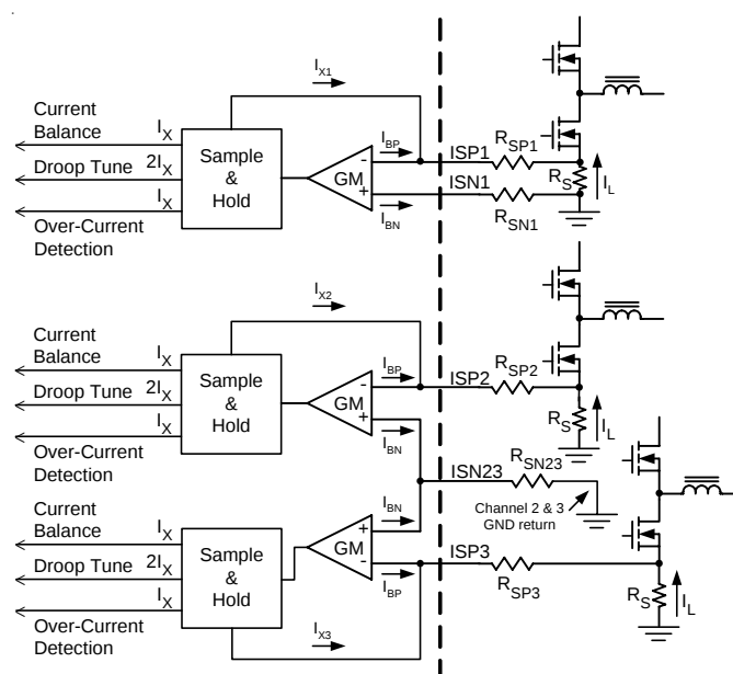
Figure 1. Current Sense Circuit
