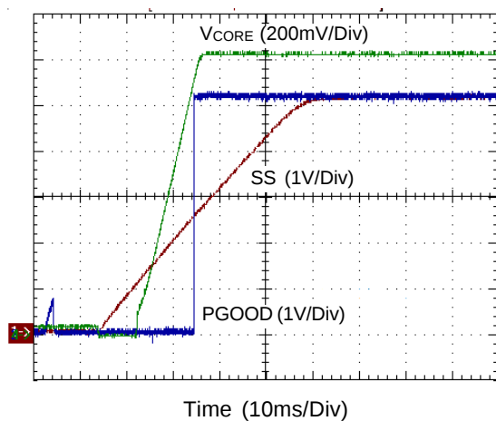
Soft Start
