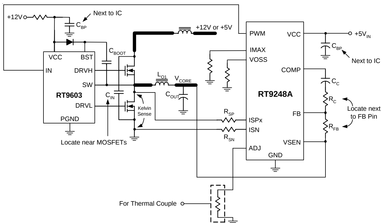
Figure 8. Layout Consideration
