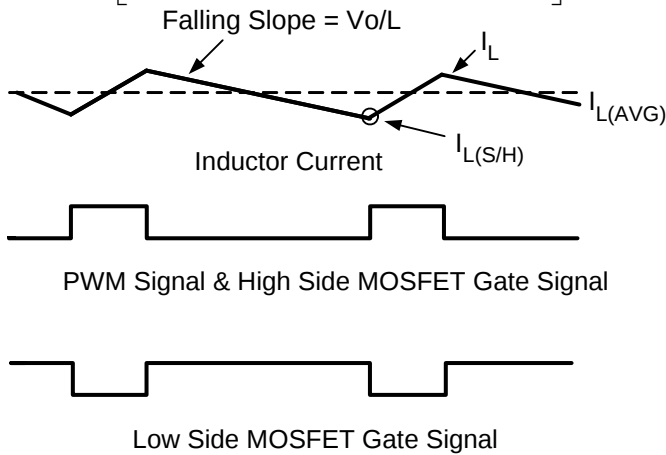
Figure 2. Inductor Current and PWM Signal
