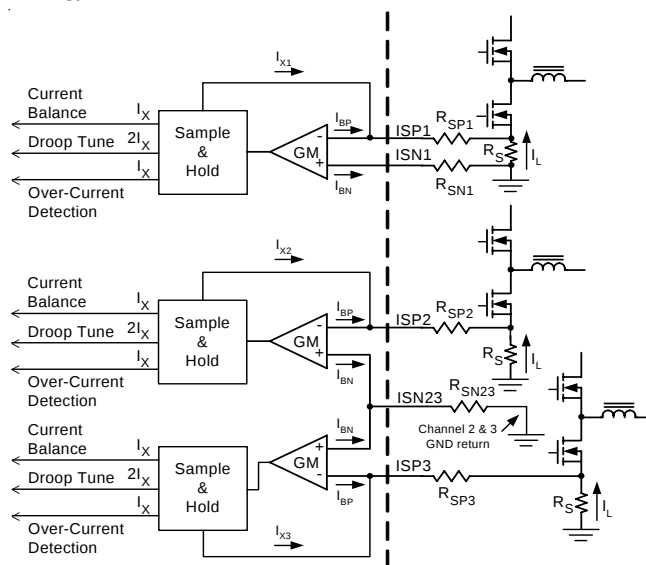
Figure 1. Current Sense Circuit
