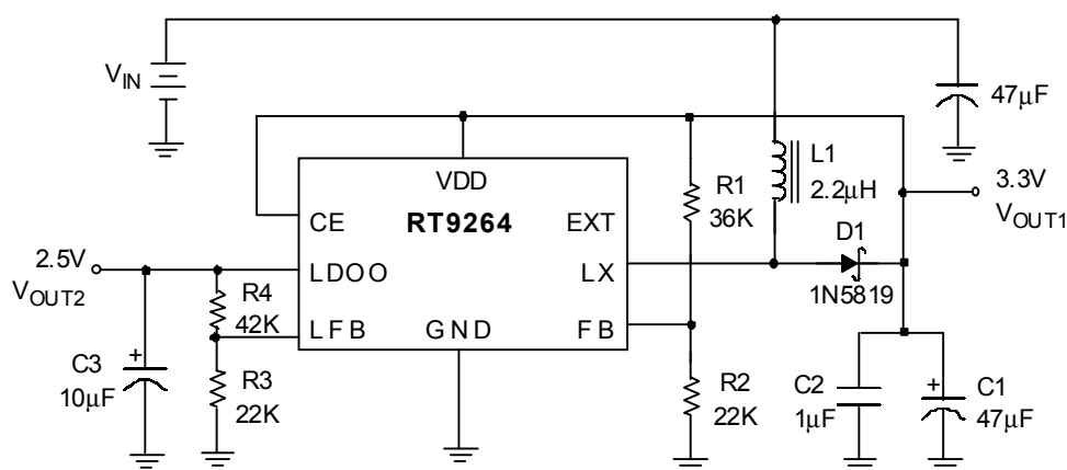
Fig. 1 RT9264 Typical Application for Portable Instruments
