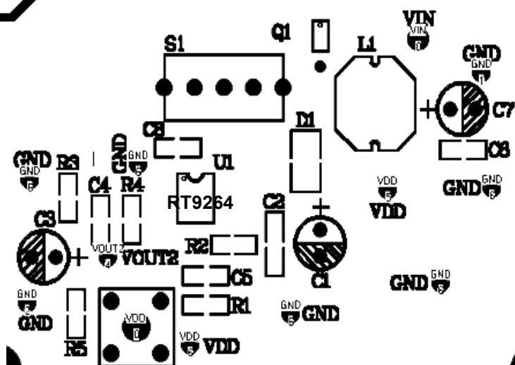
Second Layer (Full GND Plane)
