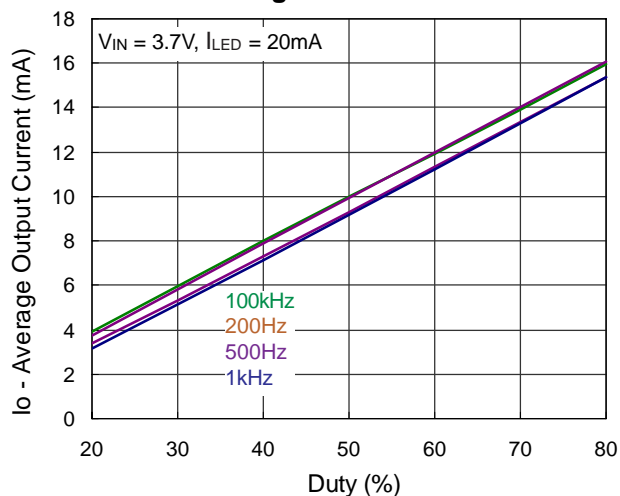
Dimming Control for 4LEDs
