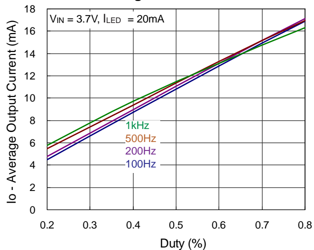
Dimming Control for 3LEDs
