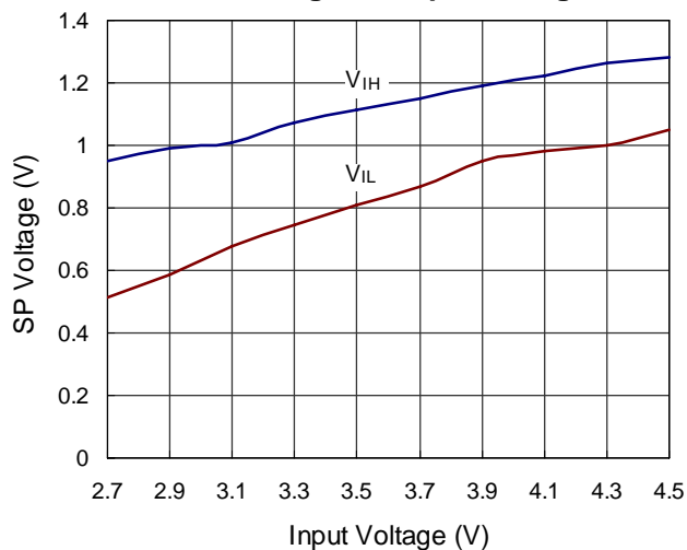
SP Voltage vs. Input Voltage
