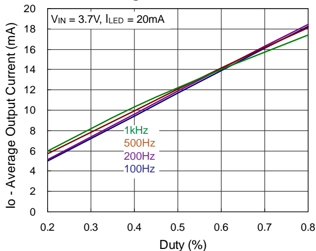
Dimming Control for 2LEDs
