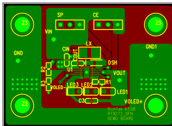
Figure 8. Top Layer
