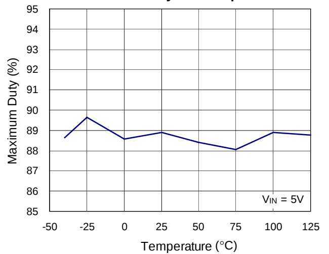
Maximum Duty vs. Temperature
