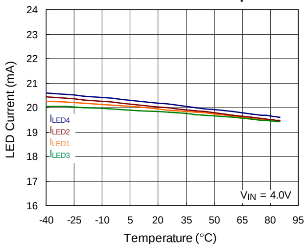
x1 Mode LED Current vs. Temperature
