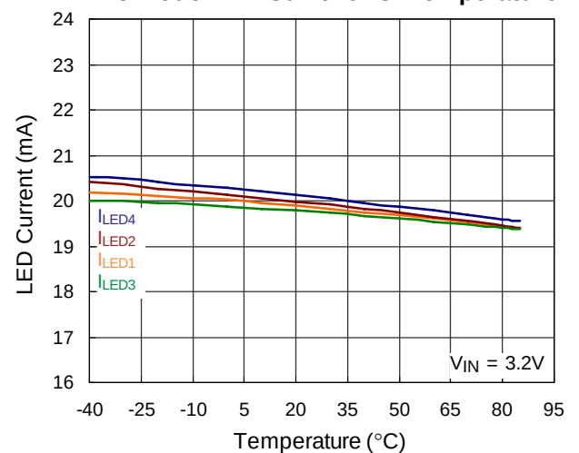
x1.5 Mode LED Current vs. Temperature
