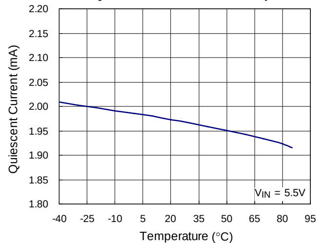
x1.5 Mode Quiescent Current vs. Temperature
