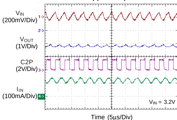
Ripple & Spike
