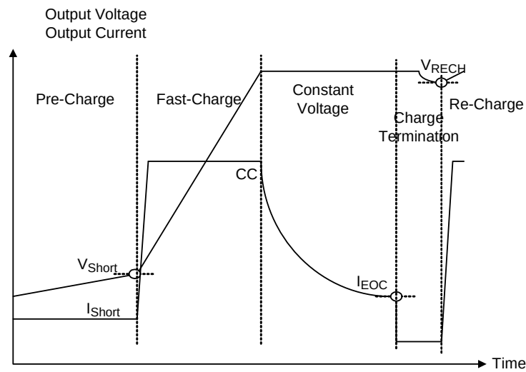
Figure 3. Charging I-V Curve
