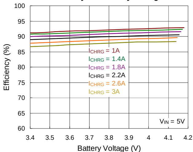
Efficiency vs. Battery Voltage
