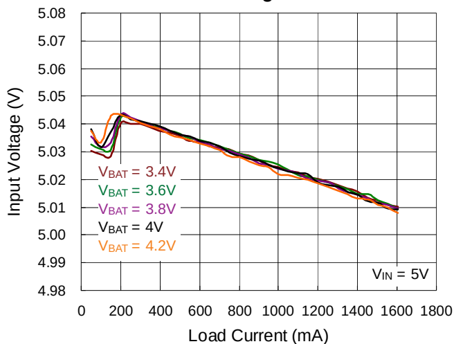
Load Regulation
