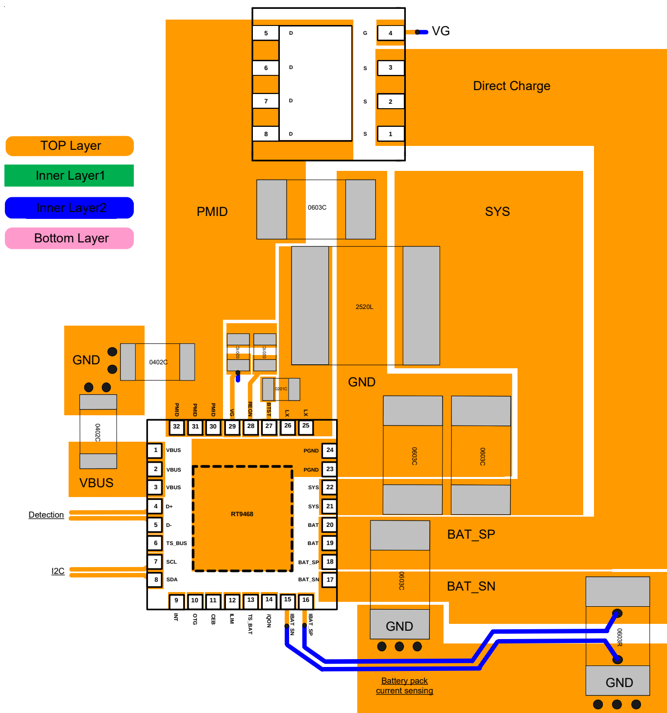
Figure 2. PCB Layout Guide
